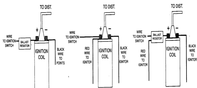
FIGURE 1 WIRING DIAGRAM CONVENTIONAL POINTS SYSTEM WITH BALLAST RESISTOR
